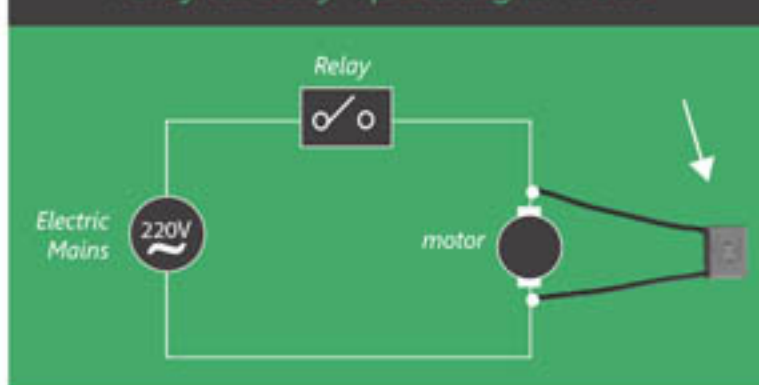
Relay directly operating a motor
