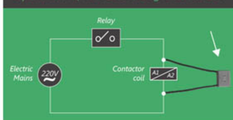
Operation of the load using a contactor
