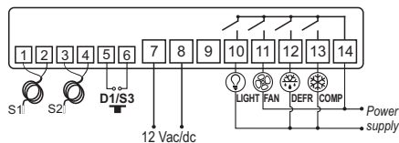
Image III - Connection 12 Vac/dc
