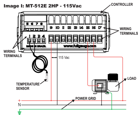
Image I: MT-512E 2HP - 115Vac
