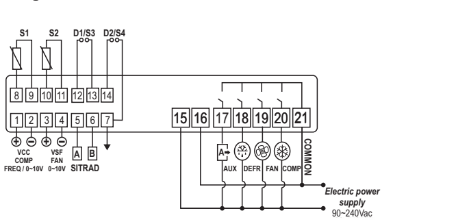
Image II - 12 Vac/dc Connection
