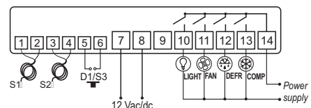
Image III - Connection 12 Vac/dc
