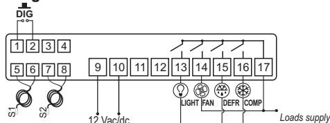
Image III - Connection 12 Vac/dc
