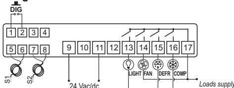
Image IV - Connection 24 Vac/dc
